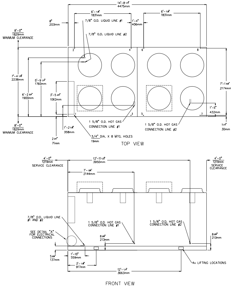
Figure DD-7 — CAUC-C80 Unit Dimensions, Recommended Clearances, Mounting Locations, Electric and Refrigerant Connection Sizes and Locations
