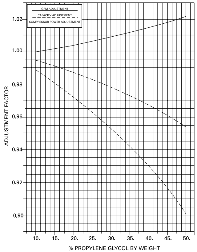
Chart PAF-4— Propylene Glycol Performance Factors
