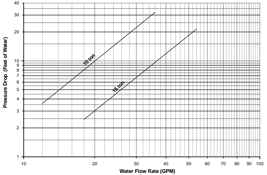
Chart PAF-1 — Evaporator Water Pressure Drop 10 and 15 Ton Air-Cooled Chillers
