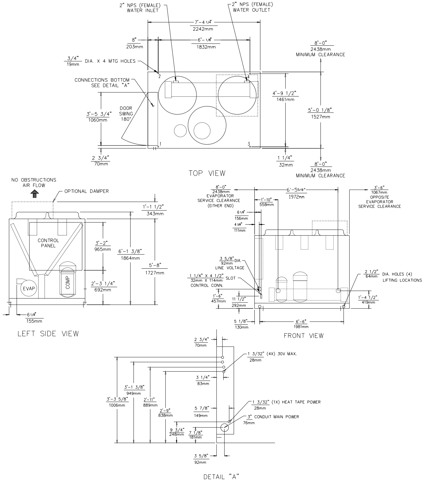
Figure DD-4 — CGAF-C25 Unit Dimensions
