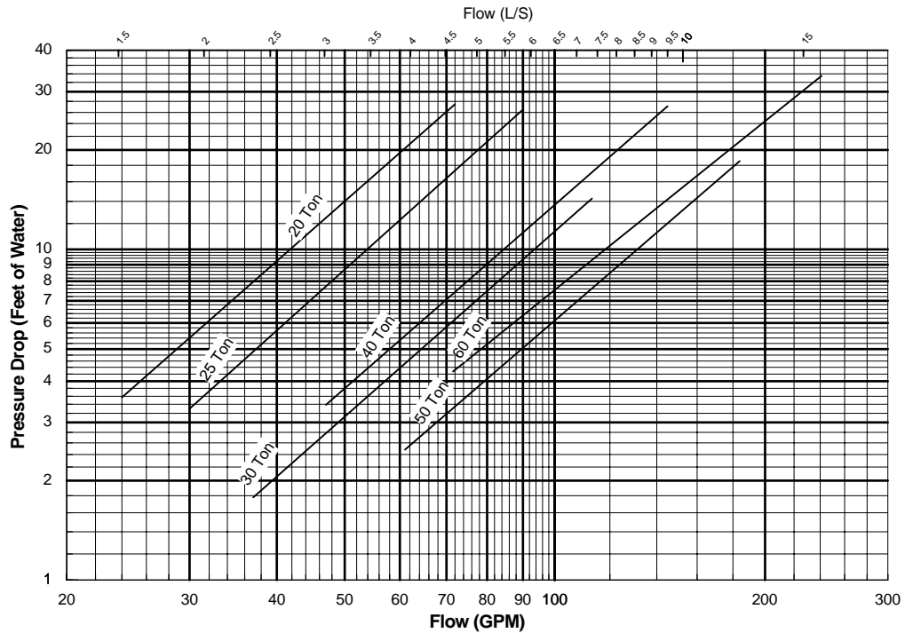
Chart PAF-2 — Evaporator Water Pressure Drop 20-60 Ton Air-Cooled Chillers
