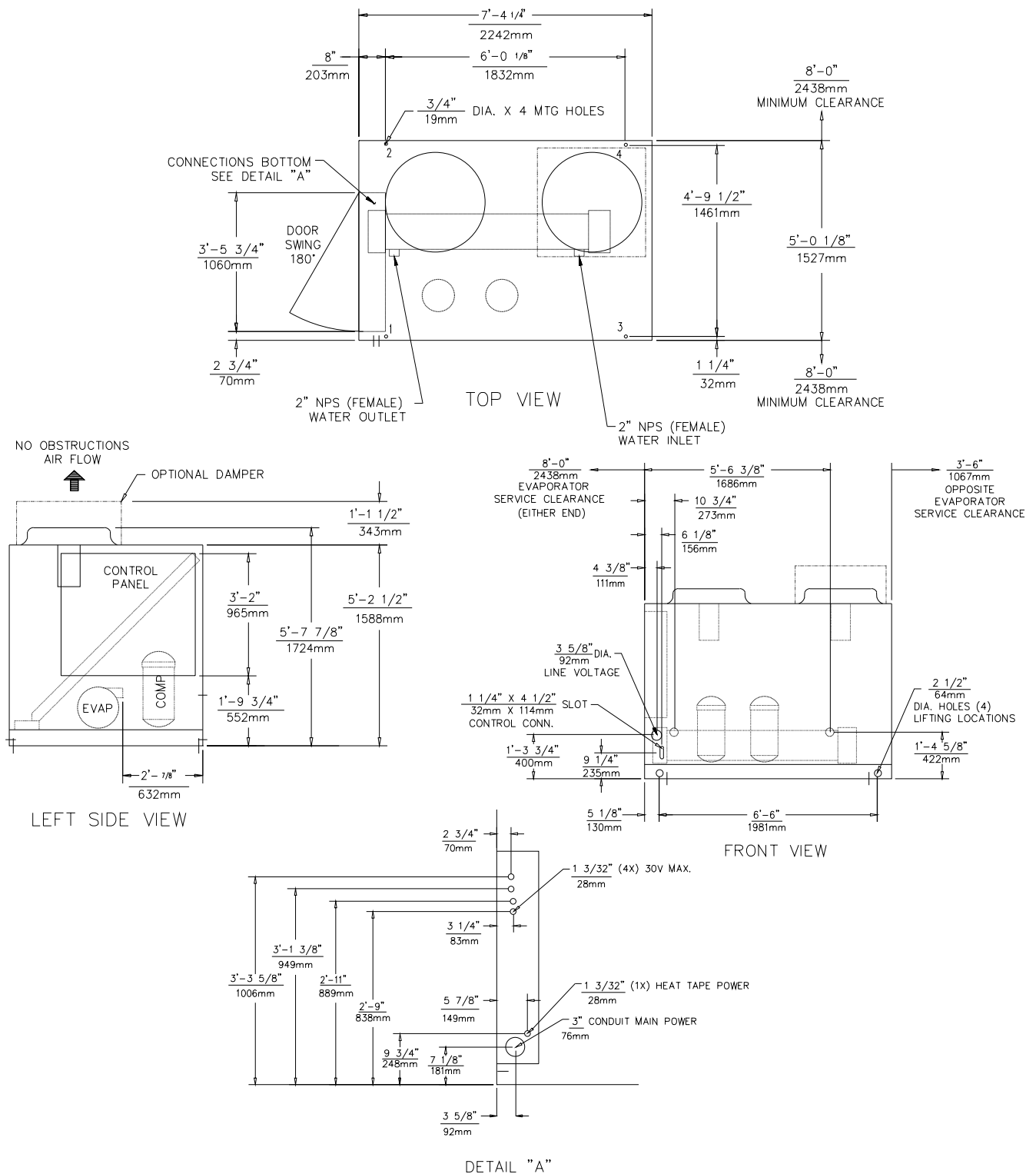
Figure DD-3 —Figure 37-1 — CGAF-C20 Unit Dimensions
